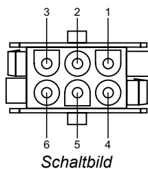
6-pin AMP Stecker
