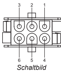
6-pin AMP Stecker
