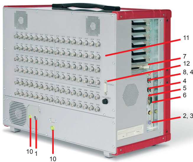
Typical DEWE-4011 rear view
