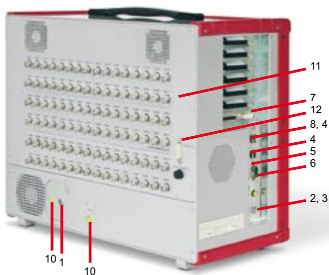
Typical DEWE-4011 rear view
