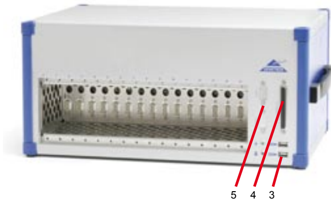
Typical DEWE-510 front view
