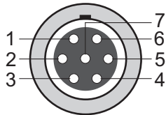
7-pin LEMO connector (female)
