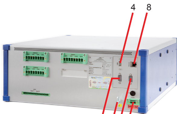
Typical PFR-821 rear view
