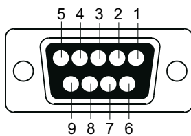
9-pin male SUB-D connector
