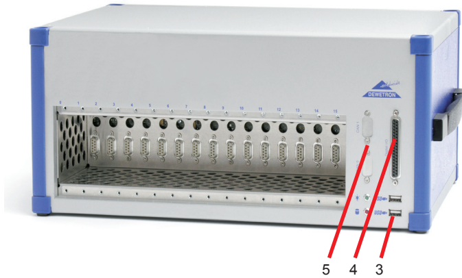
Typical DEWE-510 front view
