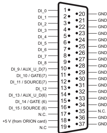
37-pin female D-SUB connector DI0 .. DI15
