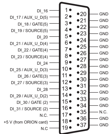
37-pin female D-SUB connector DI16 .. DI31
