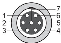
7-pin female LEMO connector EGG.1B.307 CNT0 .. CNT7
