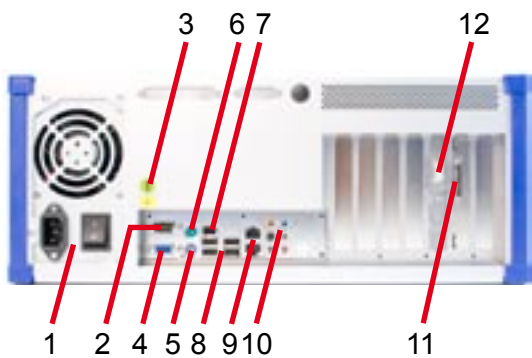
Typical DEWE-818 rear view
