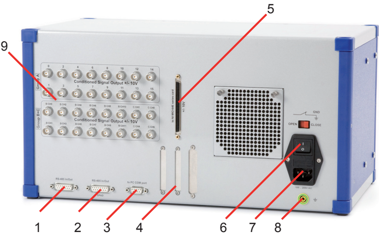
Typically DEWE-32-3216 rear view
