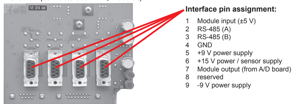
Front view (connectors for DAQ-modules)
