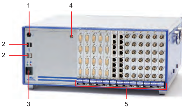
Typical DEWE2-M13 front view
