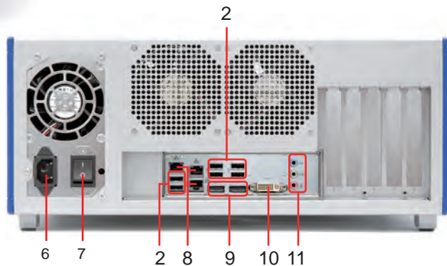
Typical DEWE2-M13 rear view
