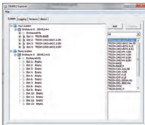
DEWE2 Explorer: Filling up of empty slots
