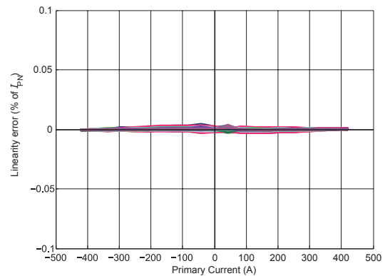
Figure 5: Linearity
