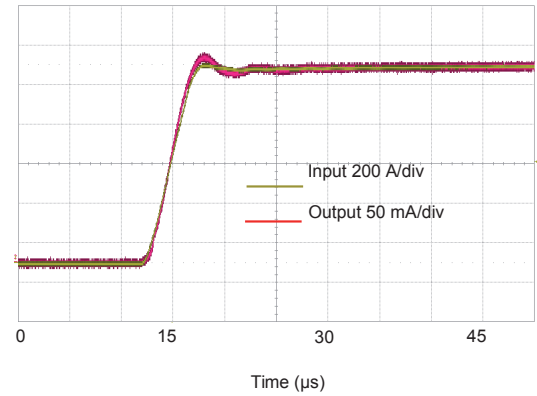
Figure 2: Typical step response (0 to 1 kA, 200 A/μs)
