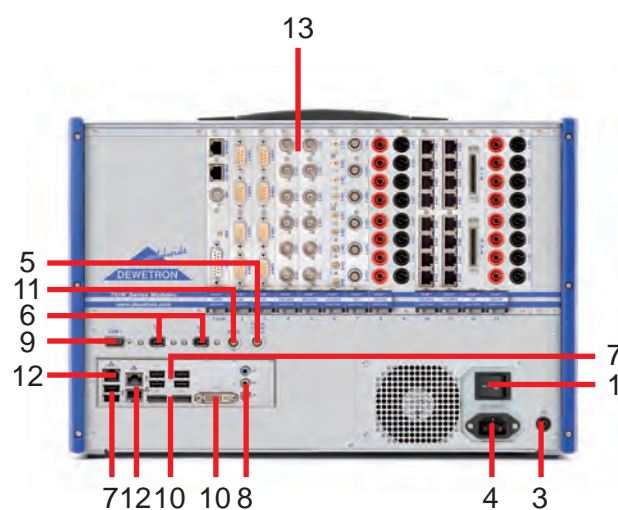
Typical DEWE2-A13 rear view
