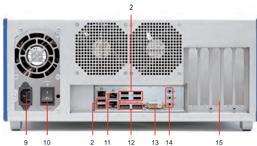
Typical DEWE2-M7 rear view
