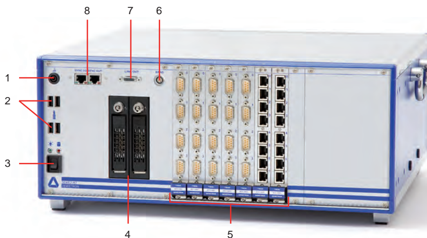
Typical DEWE2-M7 rear view
