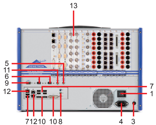
Typical DEWE2-A13 rear view
