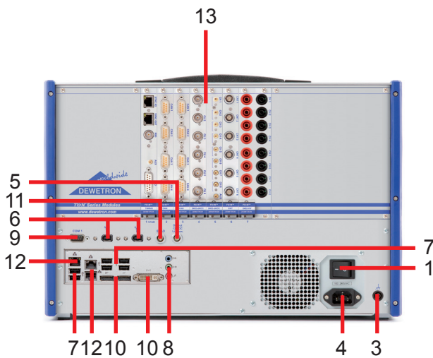
Typical DEWE2-A7 rear view
