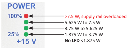
Fig. 201: +15 V / -15 V power limit
