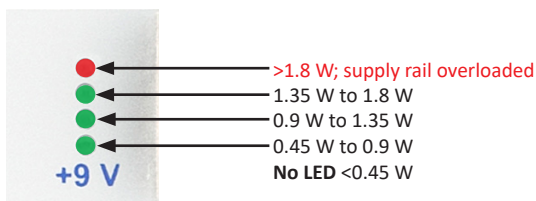
Fig. 202: +9 V power limit
