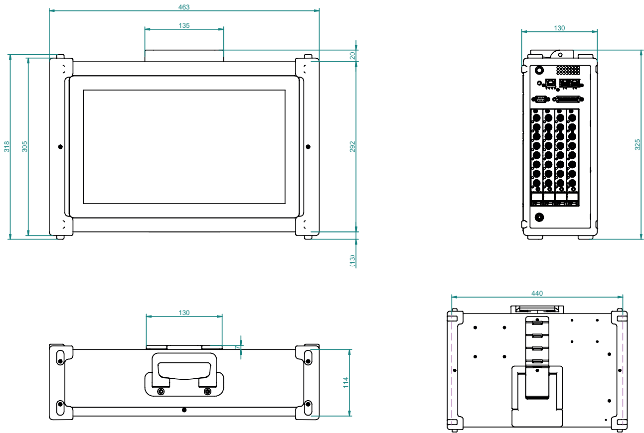
Fig. 1: Dimensions DEWE3-A4L
