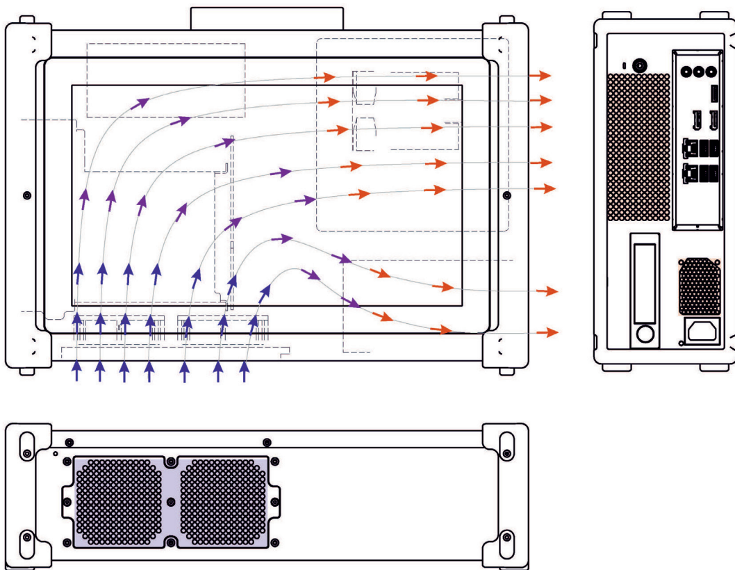
Fig. 19: Cooling concept
