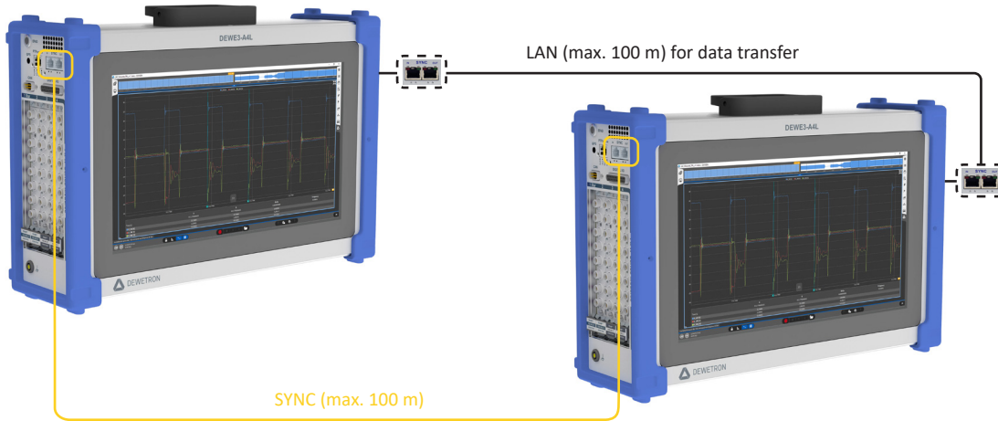
Fig. 29: Network with multiple systems
