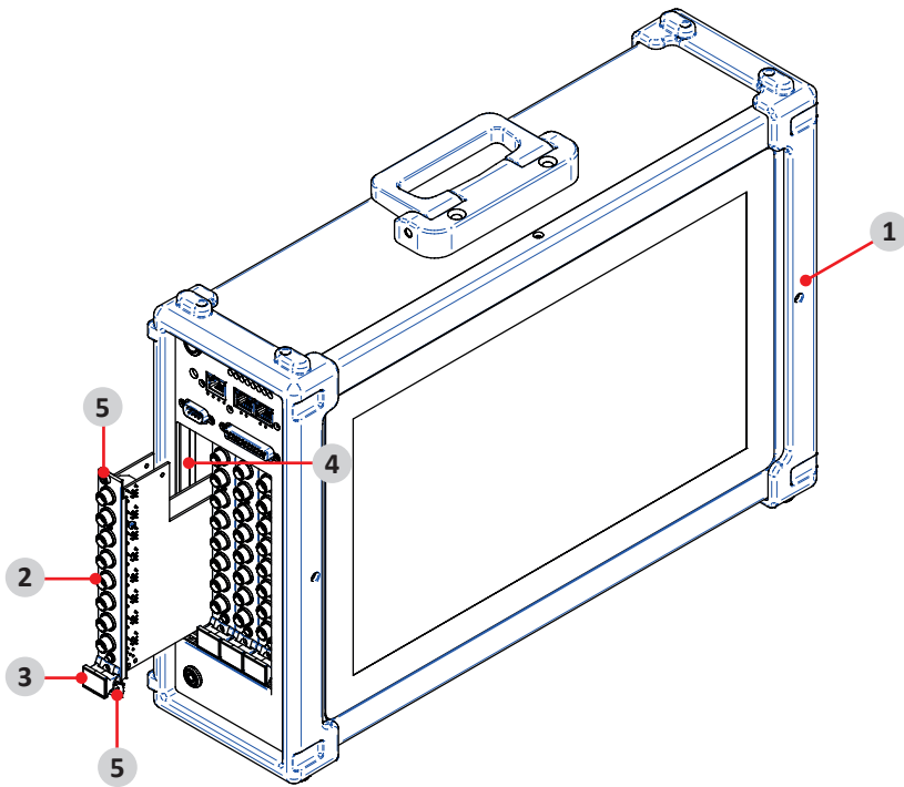
Fig. 18: Installing a TRION module
