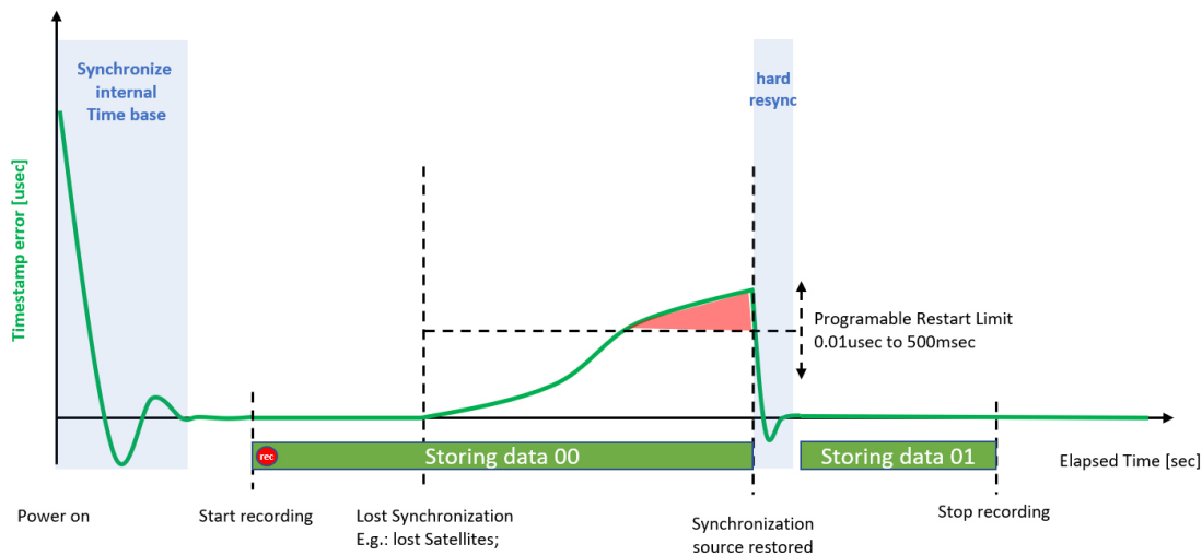
Fig. 7: Forced restart after restored synchronization
