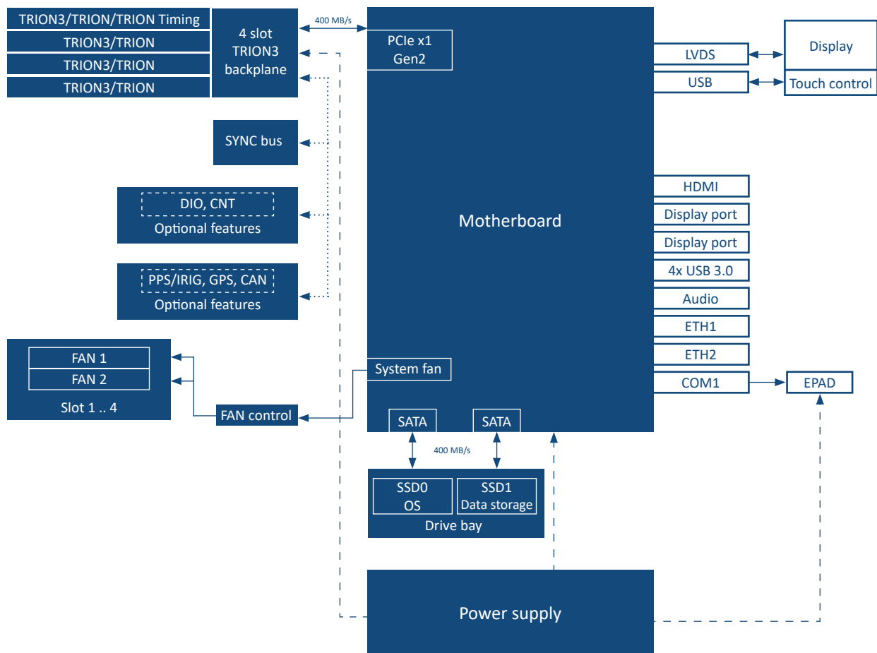
Fig. 2: Block diagram
