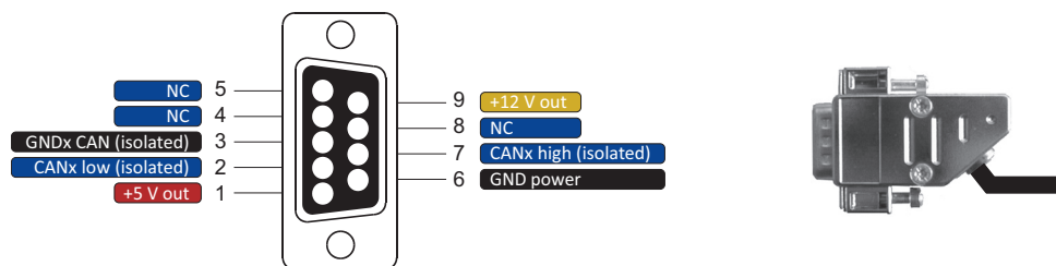
Fig. 4: D-SUB-9 CAN connector pin assignment
