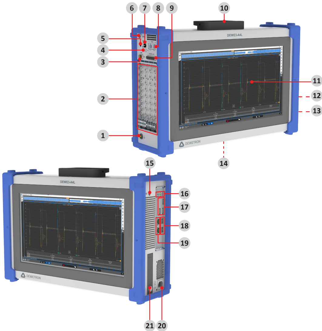
Fig. 3: DEWE3-A4L connections and ports
