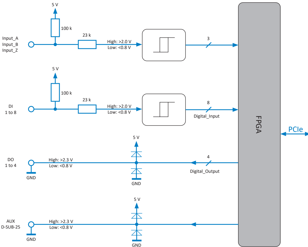
Fig. 12: Counter and digital I/O
