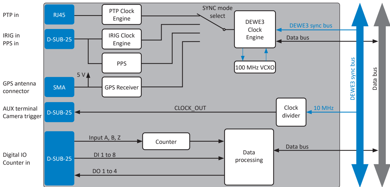
Fig. 9: Signal routing
