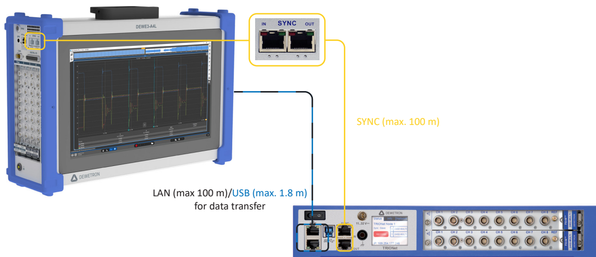
Fig. 28: Channel expansion with TRIONet
