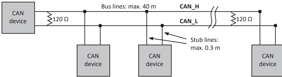
Fig. 5: Highspeed CAN
