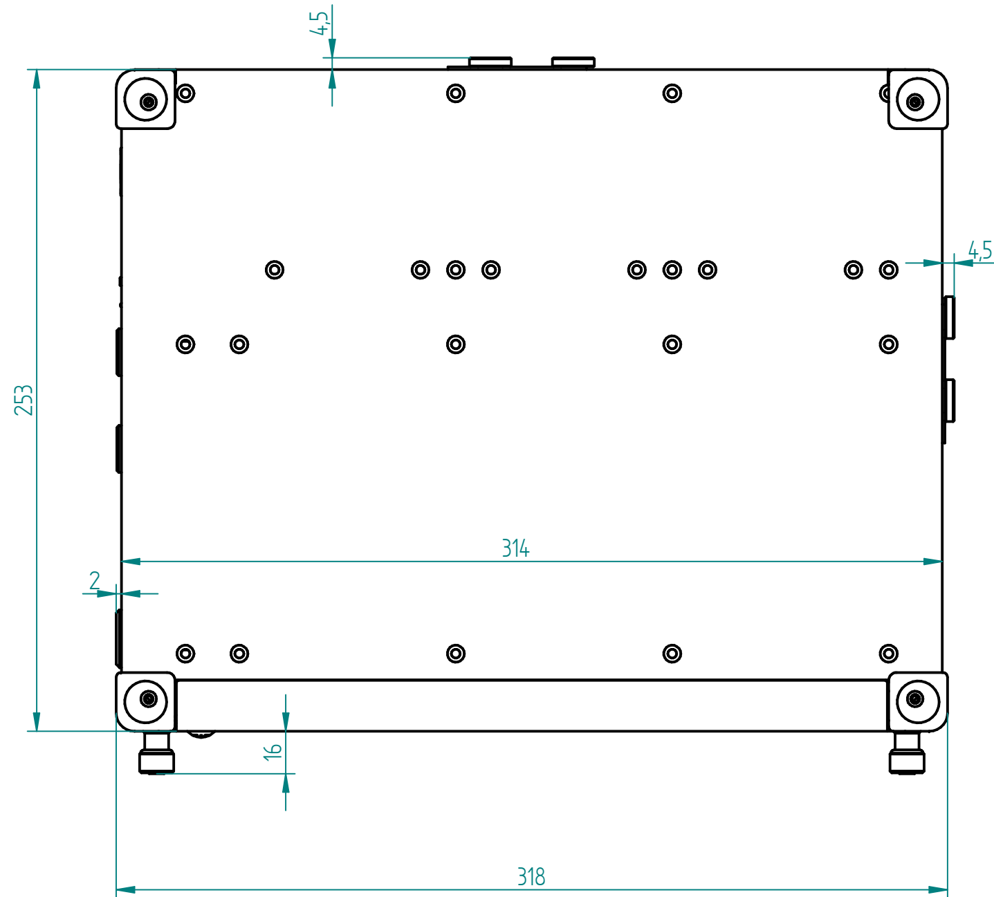
DW3-UPS-DC_Akku-Box
